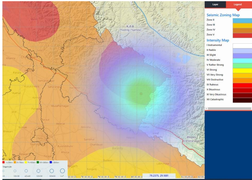
Fig 2: Map showing the intensity map of M 3.8 earthquake occurred on 22 th , January 2023 at Pithoragarh District, Uttarakhand, India.
