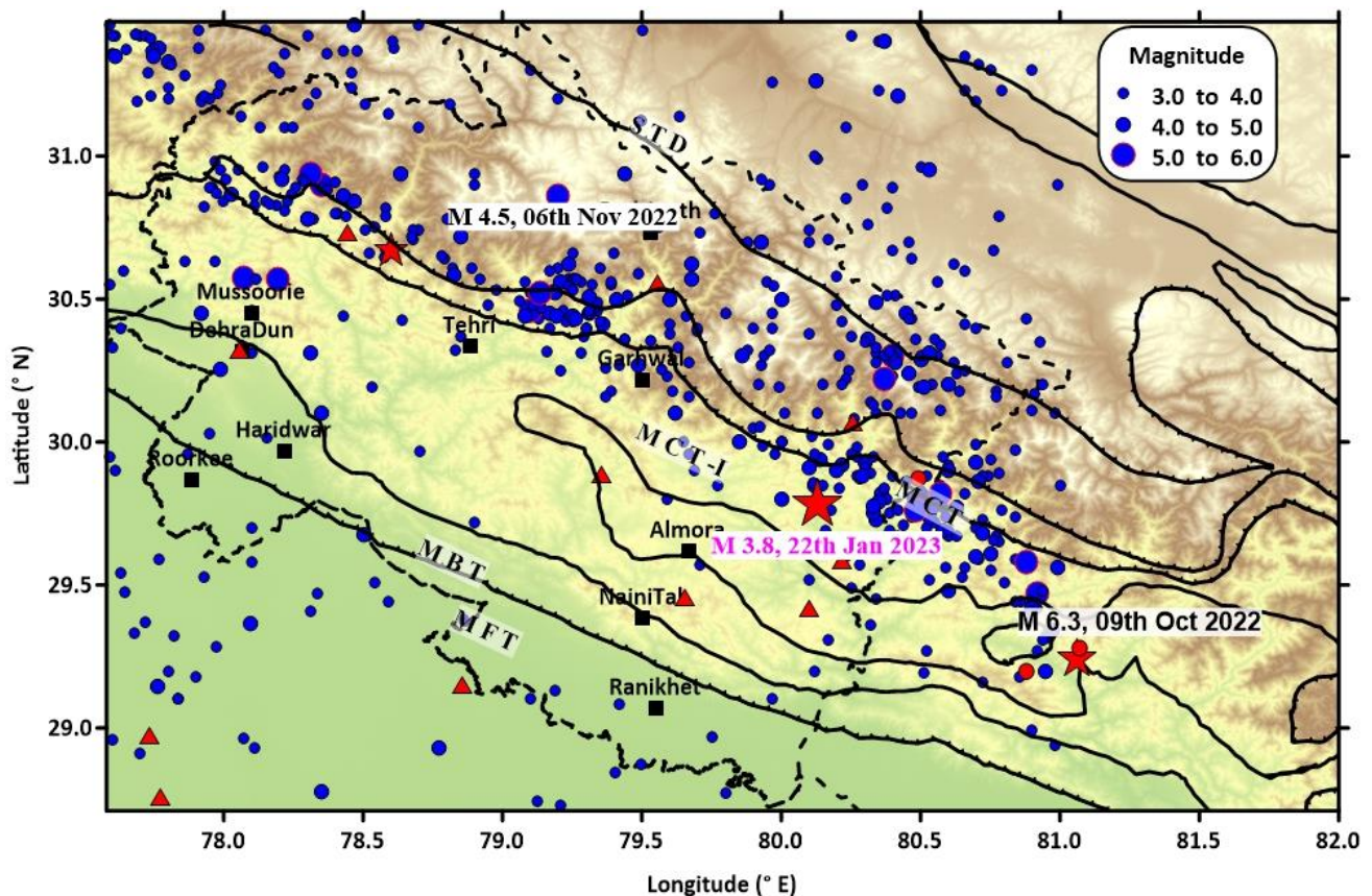
Fig 1: Map showing the location of earthquake of M 3.8 (Red Star) occurred on 22 th January 2023 at Pithoragarh District, Uttarakhand India. Seismological stations of NCS in Uttarakhand State are also shown as red triangle. The continuous thick black lines are the major fault system in the epicentral region.
