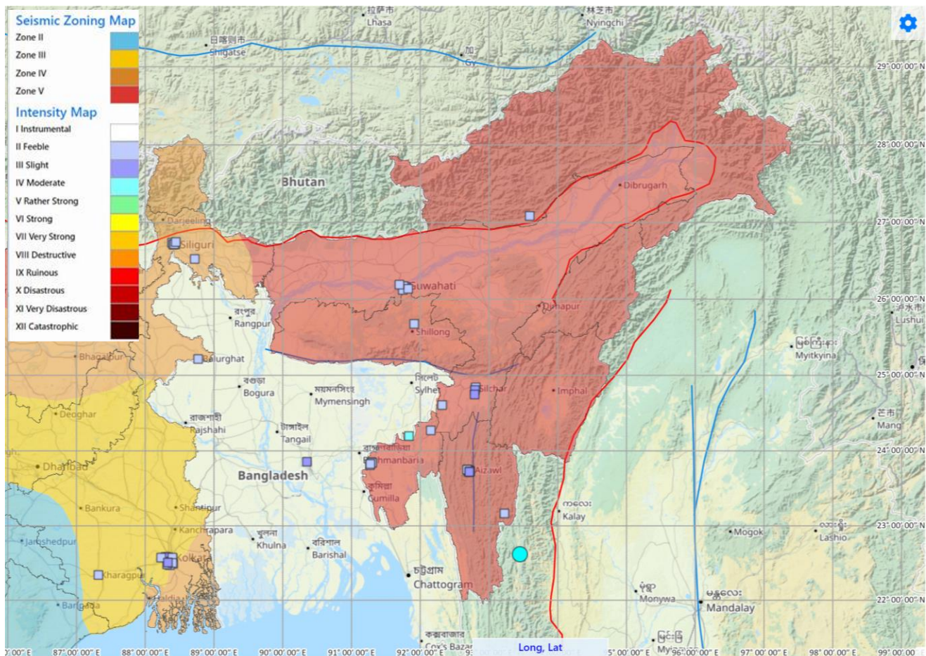
Figure-2 Felt responses received for this earthquake of M:6.2
