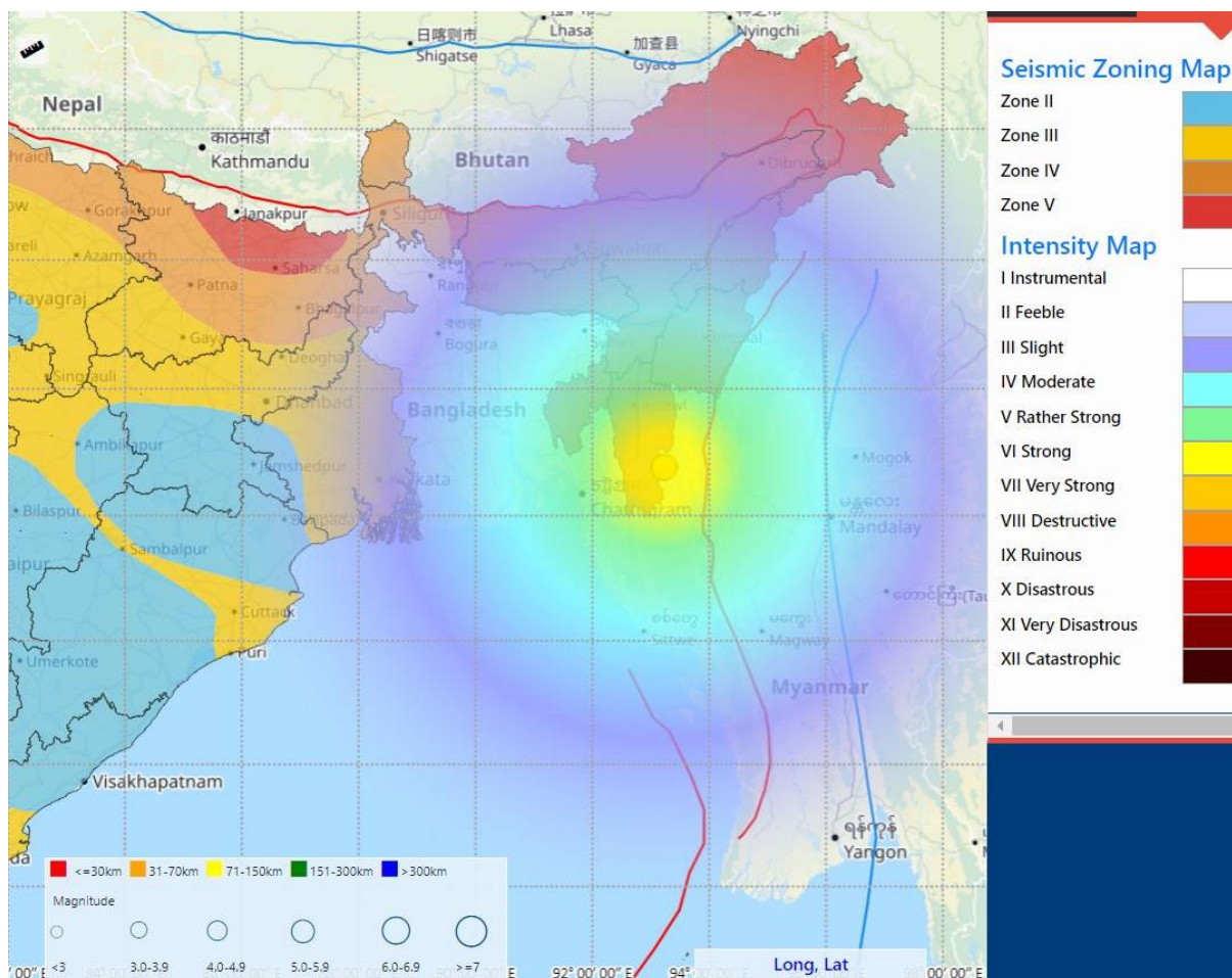
Figure-1: Location of earthquake of 26 th November, 2021 (M:6.2), Epicenter of earthquake is in Myanmar.
