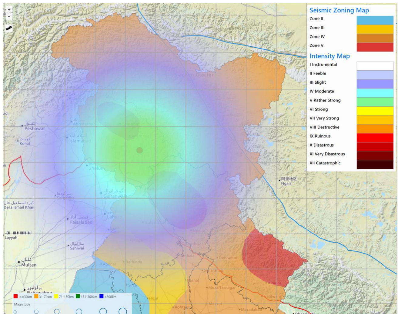
Fig.1: Location and expected intensity of earthquake occurred on 11 th January 2021.
